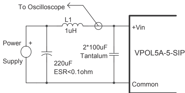
Figure 10. Input Reflected-Ripple Test Setup
