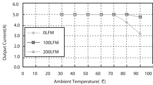
Figure 2. Typical Power De-rating for 5V IN 3.3Vout
