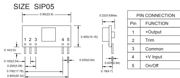
Figure 14 VPOL5A-5-SIP Mechanical Outline Diagram
