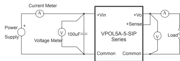
Figure 11. VPOL5A-5-SIP Series Test Setup
