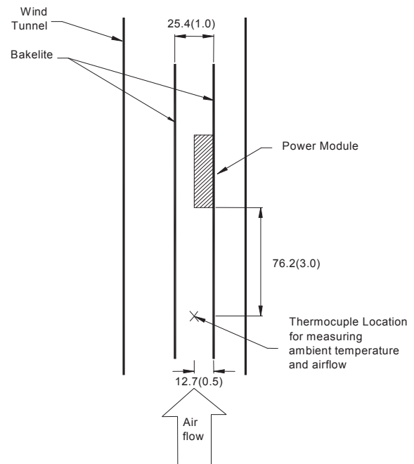
Note : Dimensions are in millimeters and (inches) Figure 6. Thermal Test Setup
