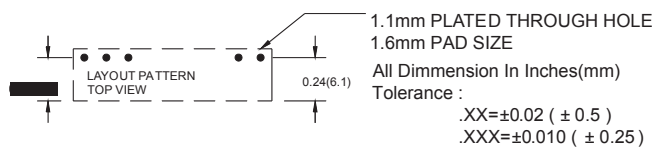
Figure 5. Recommended SIP Footprint
