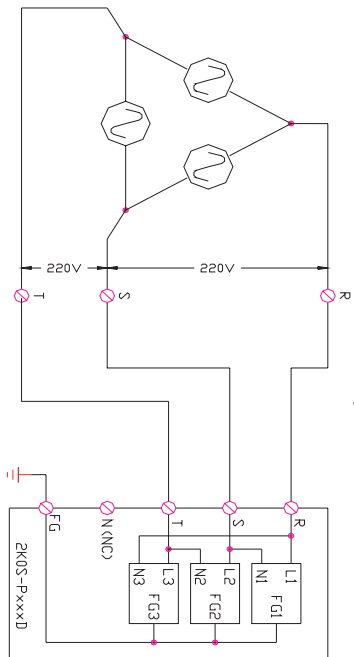
FIG. C: 3Ø 3W 220VAC SYSTEM
