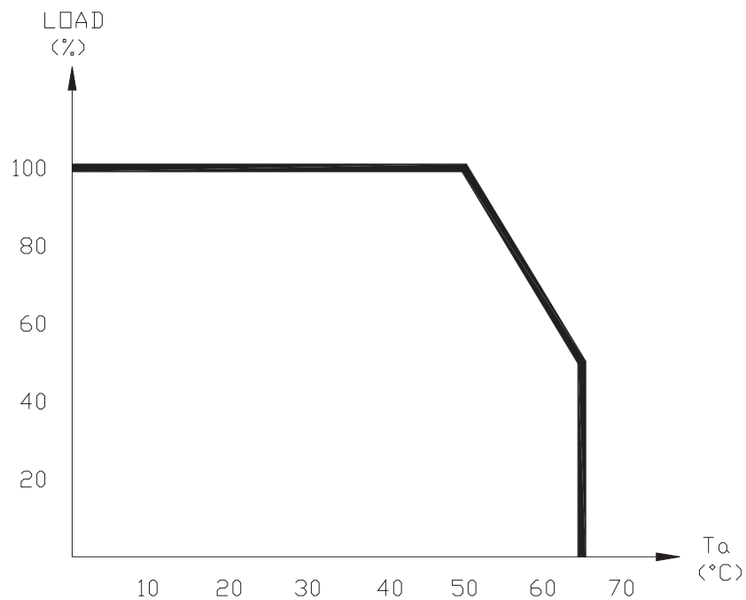
Derating Curve
