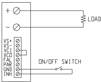
ON/OFF CONTROL BY SWITCH
