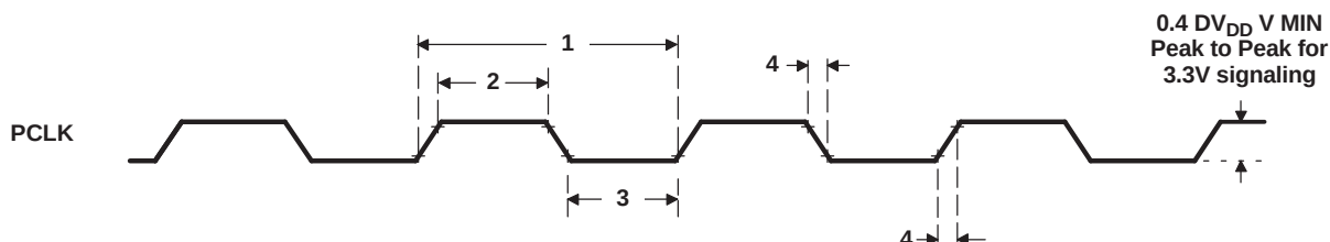
Figure 5-46. PCLK Timing
