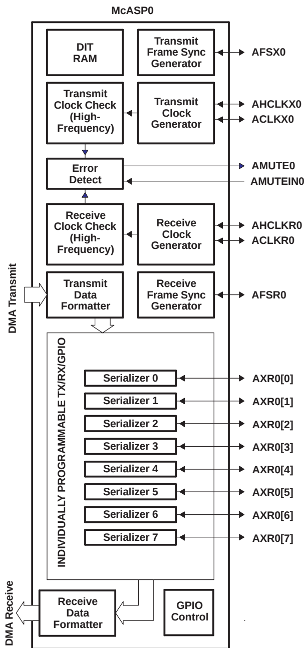
Figure 5-32. McASP0 Configuration
