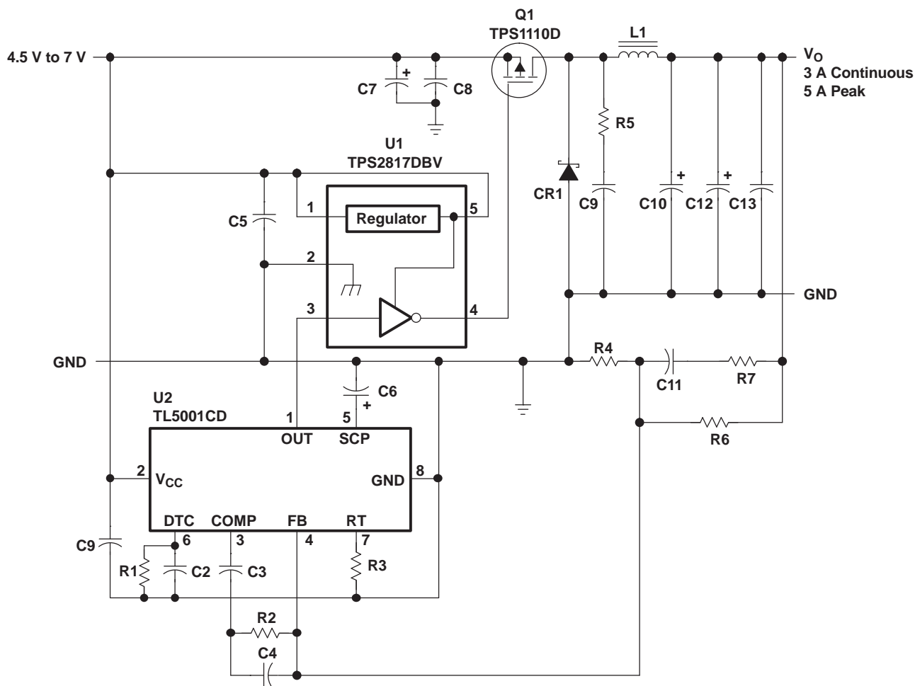
Figure 23. Step-Down Application
