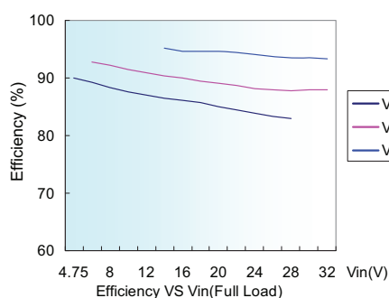
Efficiency
