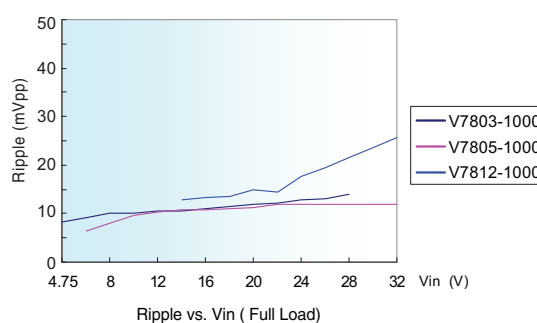
Output Ripple
