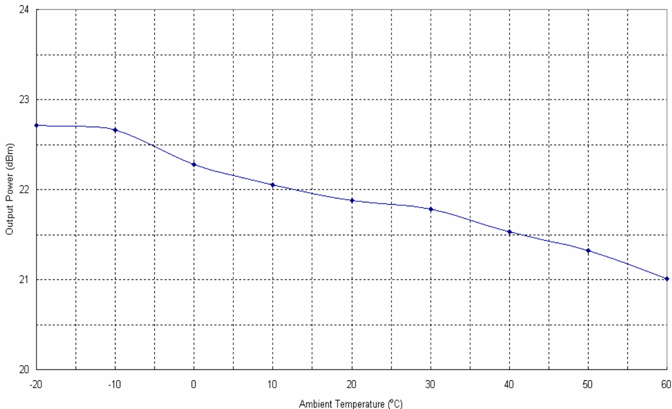
Output Power Vs Temperature
