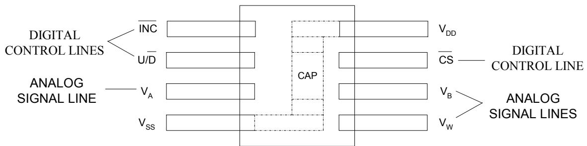
FIGURE 9 – WMS7140/1 LAYOUT
