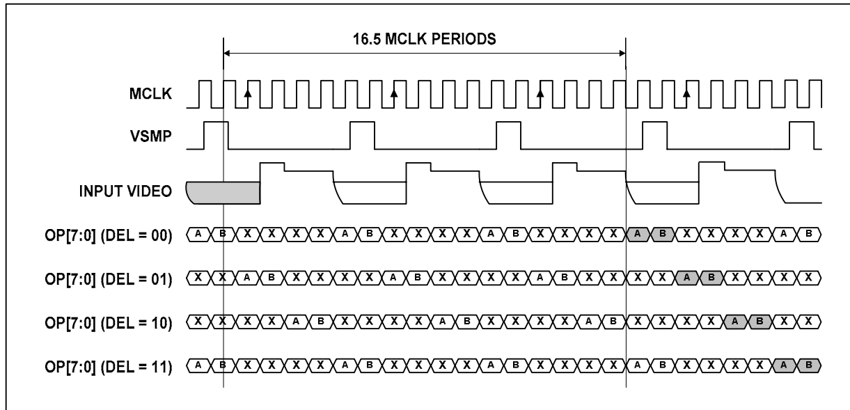
Figure 24 Mode 2 Operation
