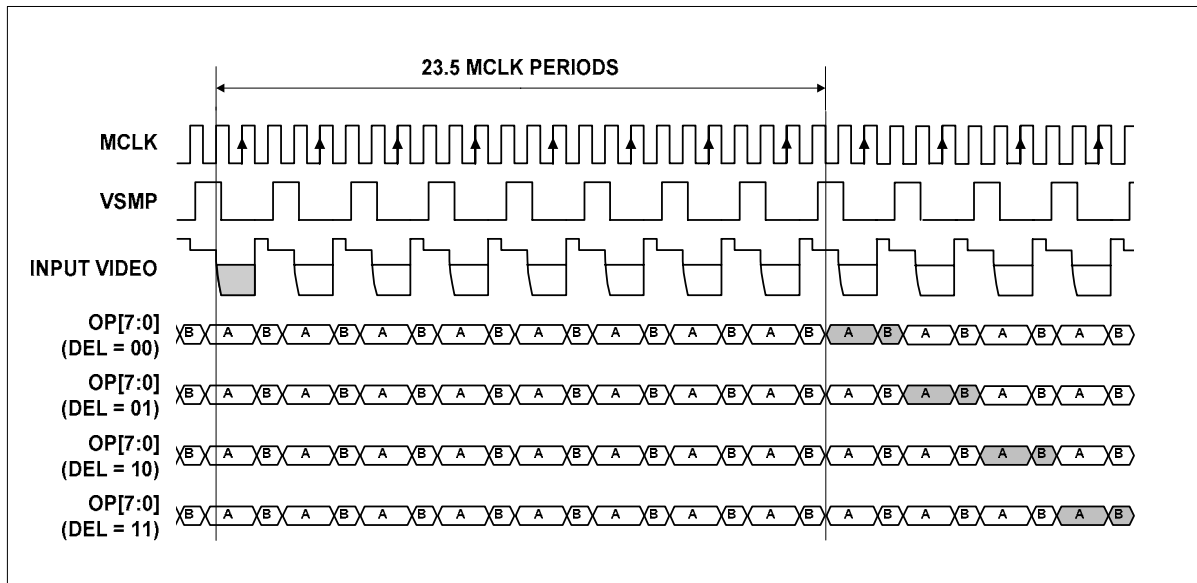
Figure 25 Mode 3 Operation
