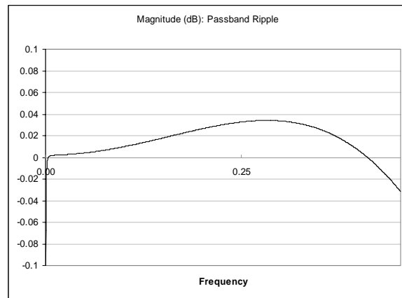
Figure 61 ADC Digital Filter Ripple
