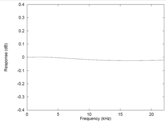
Figure 59 De-Emphasis Error (44.1KHz)
