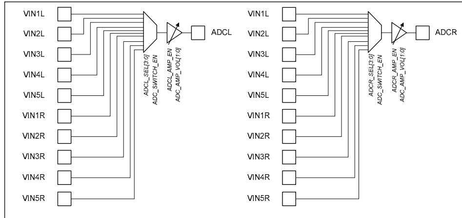
Figure 20 ADC Input Selector Control
