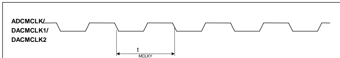
Figure 1 MCLK Timing
