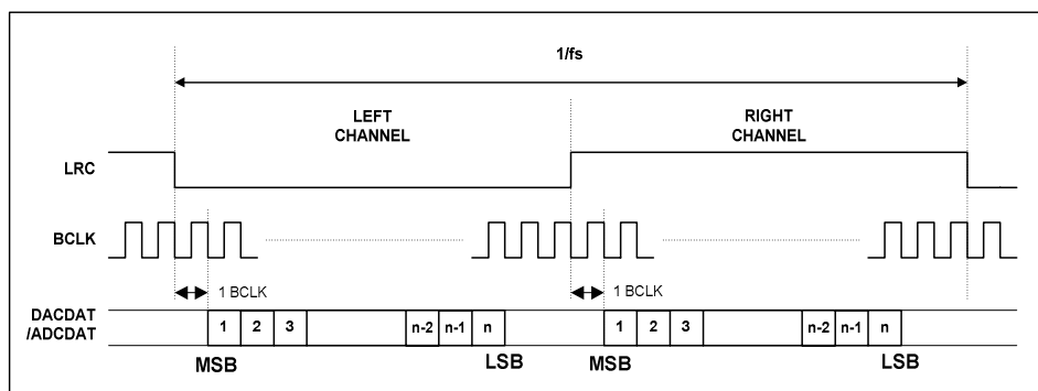
Figure 33 I^2S Audio Interface (assuming n-bit word length)
