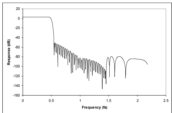
Figure 42 DAC Digital Filter Frequency Response (64xOSR)
