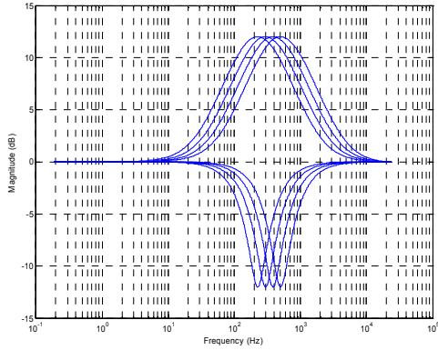
Figure 52 EQ Band 2 - Peak Filter Centre Frequencies, EQ2BW=0
