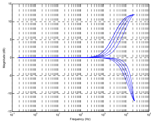
Figure 61 EQ Band 5 High Frequency Shelf Filter Cut-offs
