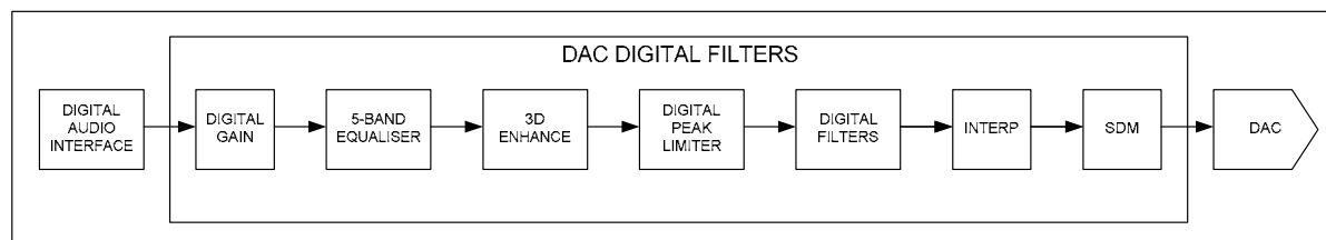
Figure 19 DAC Digital Filter Path
