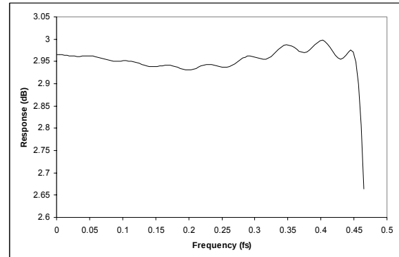
Figure 37 DAC Digital Filter Ripple (128xOSR)
