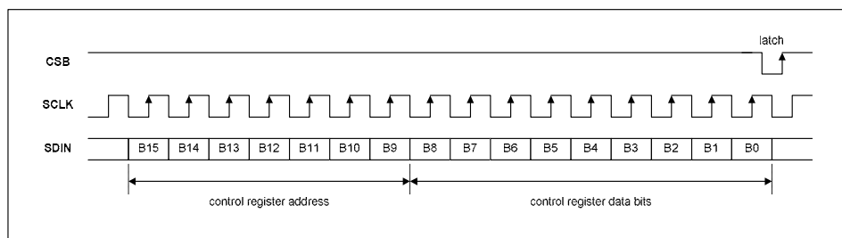
Figure 34 3-Wire Serial Control Interface
