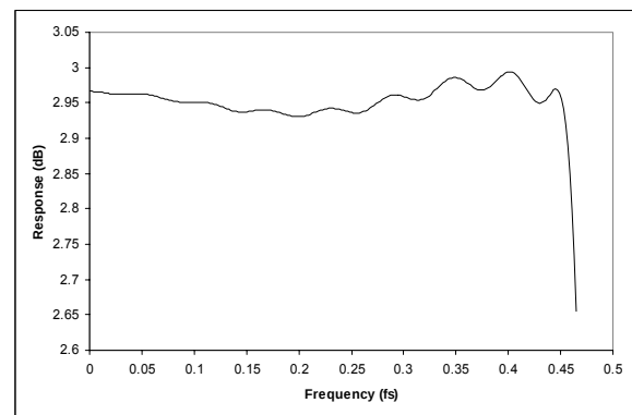
Figure 39 DAC Digital Filter Ripple (64xOSR)
