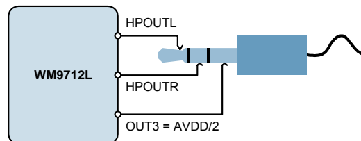
Figure 26 Capless Headphone Output Circuit Diagram (OUT3SRC = 10)
