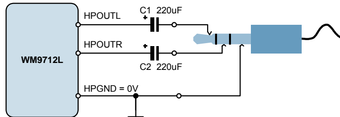
Figure 25 Simple Headphone Output Circuit Diagram
