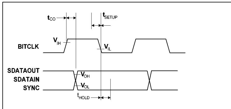
Figure 21 Data Setup and Hold (50pF External Load)
