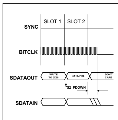
Figure 23 AC-Link Powerdown Timing
