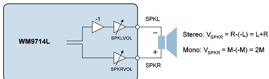
Figure 30 Speaker Output Connection (INV = 1)
