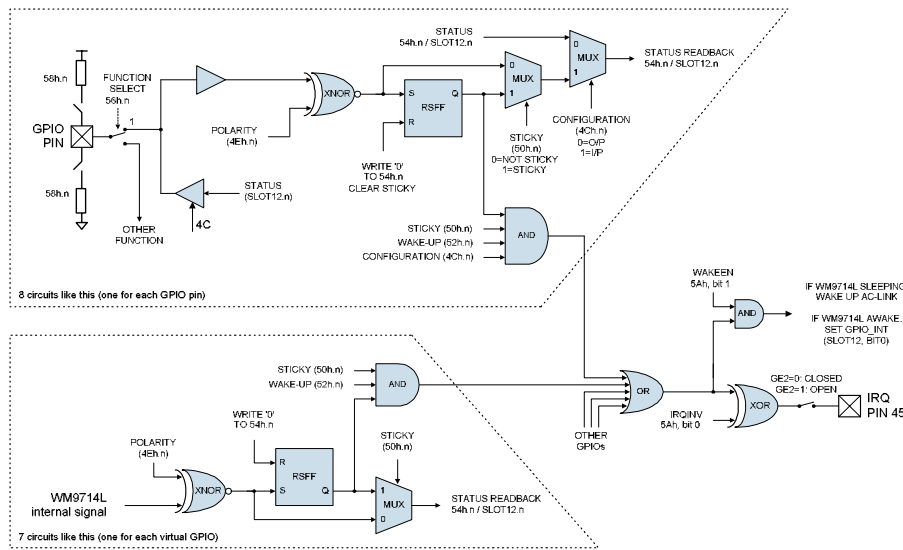
Figure 19 GPIO Logic
