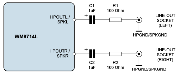
Figure 27 Recommended Circuit for Line Output
