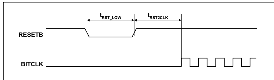
Figure 24 Cold Reset Timing
