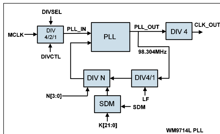
Figure 3 PLL Architecture
