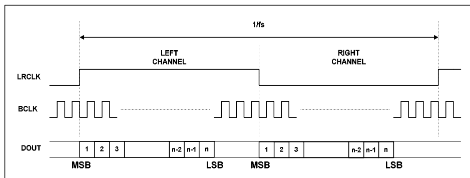
Figure 18 Left Justified Audio Interface (assuming n-bit word length)
