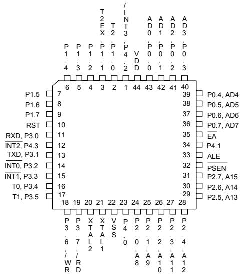
44-Pin PLCC
