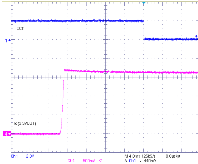
Fig.9 OC# Response When 3.3VOUT Power Into A Short
