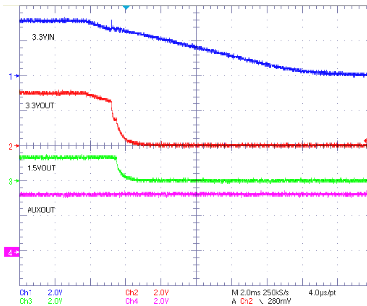
Fig.6 Output Voltage When 3.3VIN Is Removed
