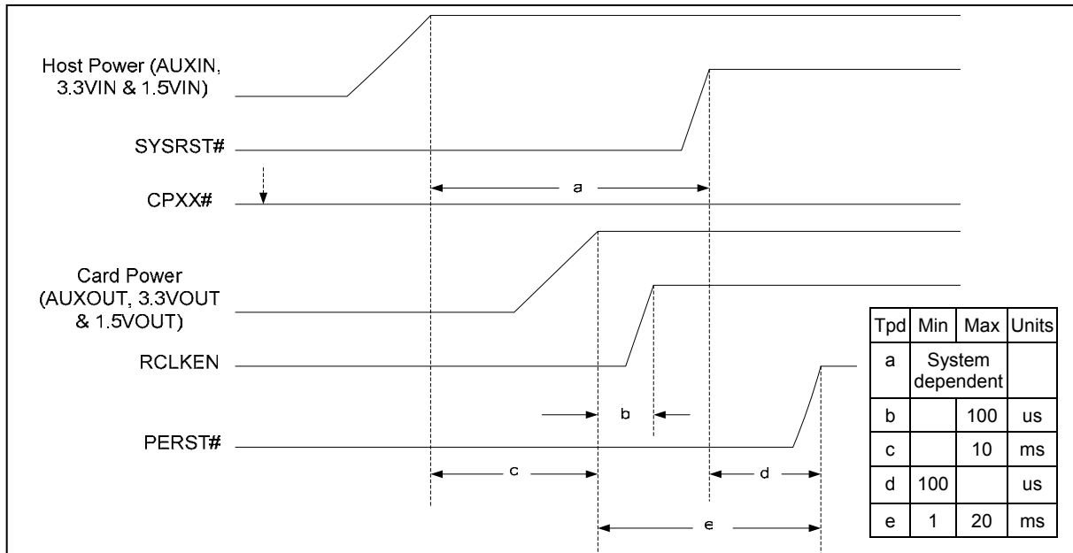
Fig.11 Card Present Before Host Power (Note.1)
