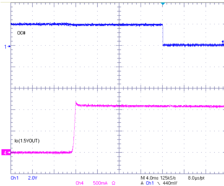
Fig.10 OC# Response When 1.5VOUT Power Into A Short
