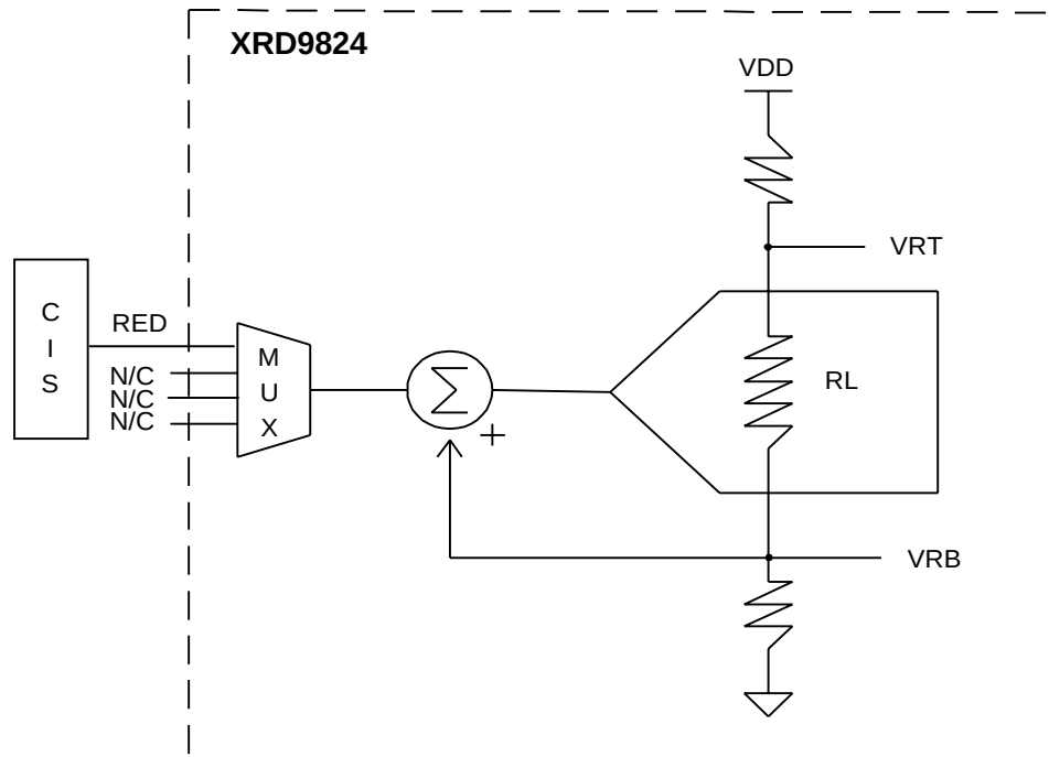
Figure 3. Application with Offset in the Range (-100mv to 500mv)
