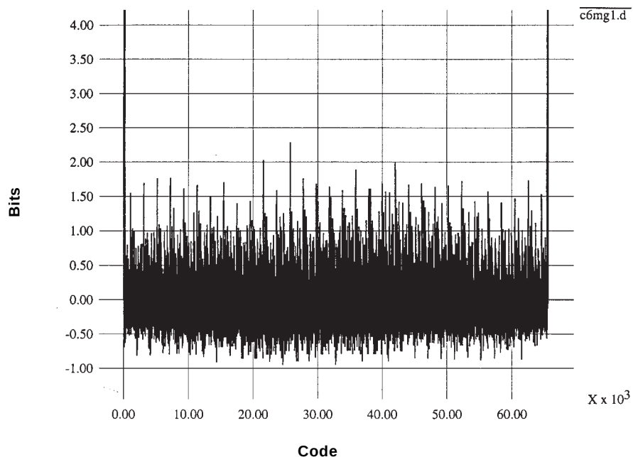
XRD9825ACD 1-channels CCD AC mode, Gain at 1A_{DD}=DV_{DD}=5.0V , Clock rate at 12MHz (16-Bit data)
