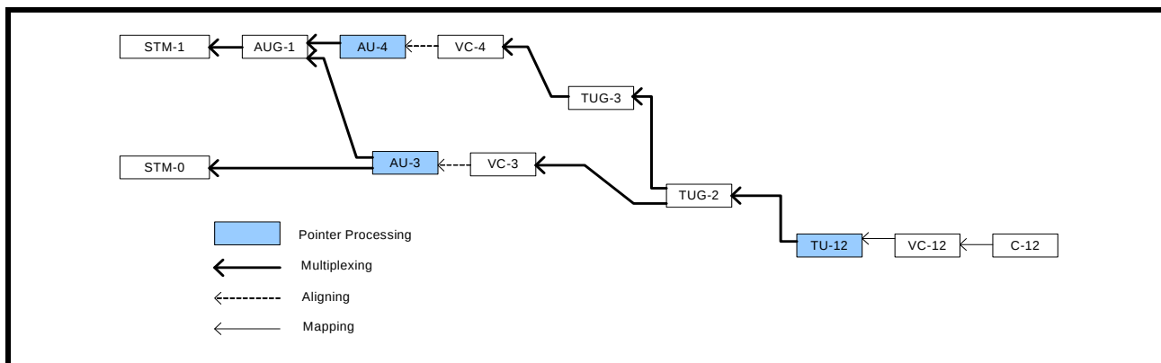
FIGURE 12. MULTIPLEXING STRUCTURE
