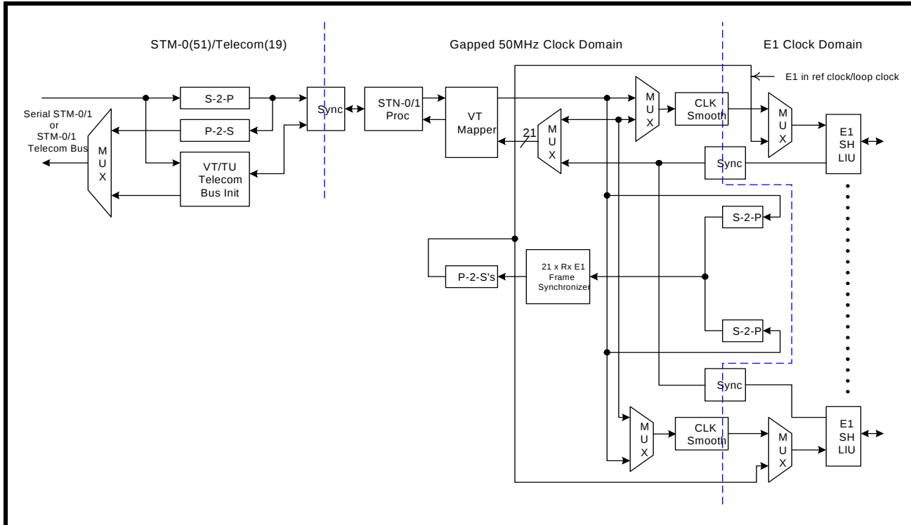
FIGURE 11. VOYAGER-LITE ARCHITECTURE
