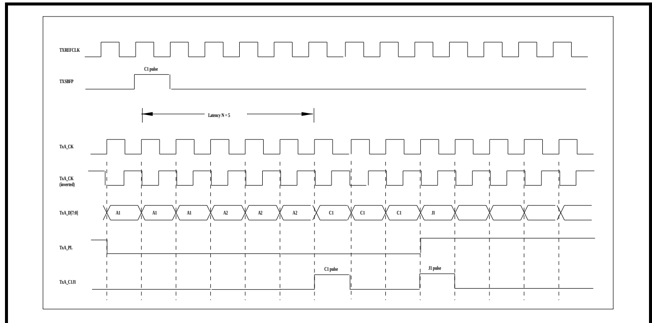
FIGURE 24. TRANSMIT TELECOM BUS INTERFACE TIMING
