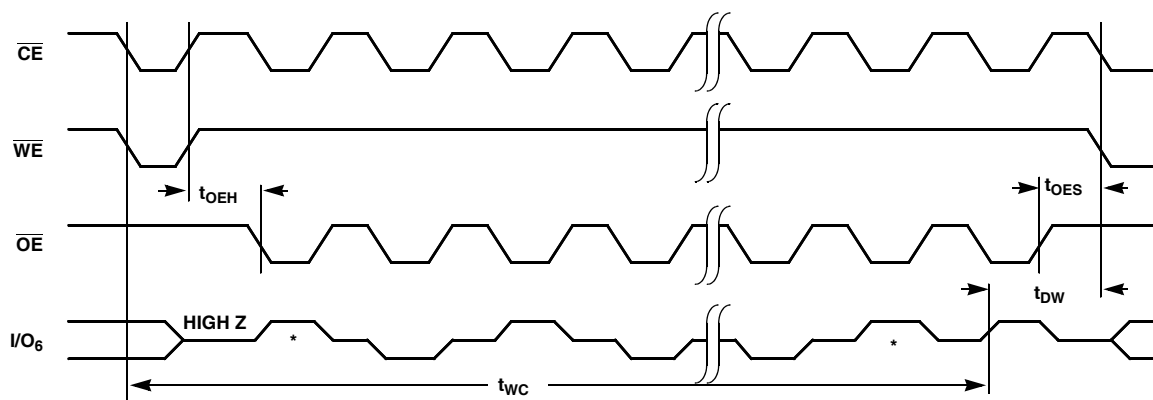
Toggle Bit Timing Diagram (Note 11)
