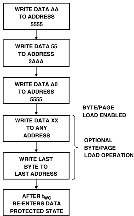
FIGURE 7. WRITE SEQUENCE FOR SOFTWARE DATA
