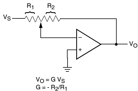
INVERTING AMPLIFIER
