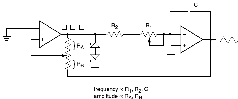
FUNCTION GENERATOR
