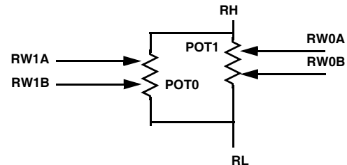
Four-Wiper DCP
