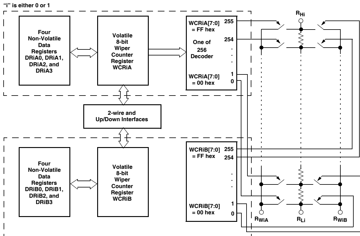
FIGURE 1. DETAILED BLOCK DIAGRAM OF ONE DCP
