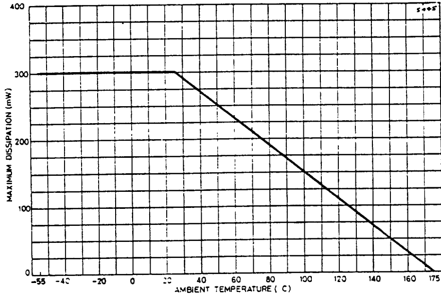
DERATING CURVE
