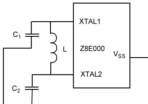
Figure 17. LC Clock
