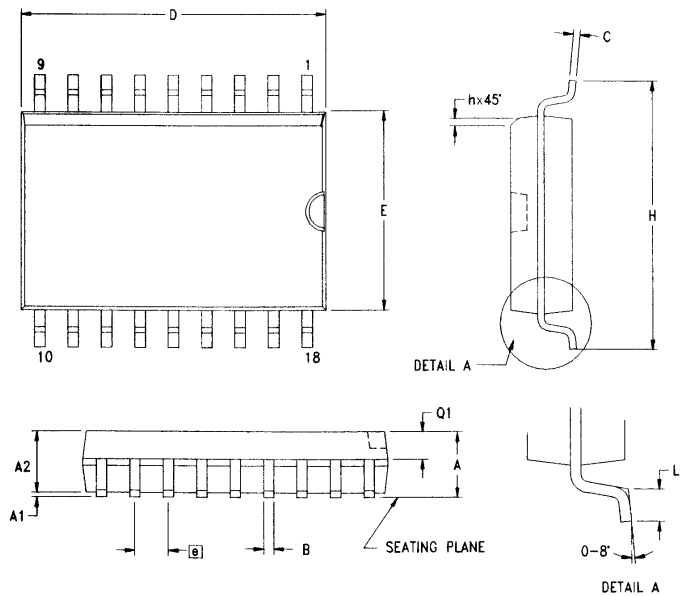
Figure 40. 18-Pin SOIC Package Diagram
