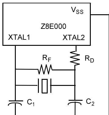
Figure 16. Crystal/Ceramic Resonator Oscillator
