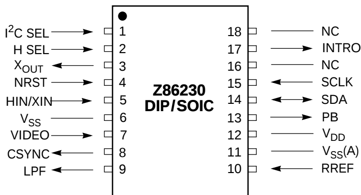
FIGURE 3. 18-PIN DIP AND SOIC DEVICES
