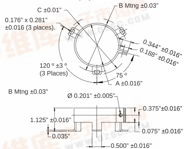
VR6, 8, 10 & 12
