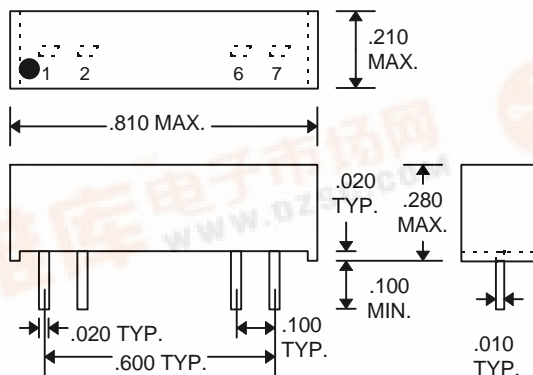
Package Dimensions
