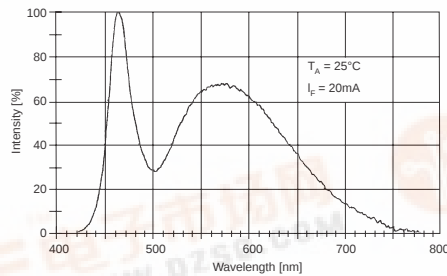
*typical luminous spectrum
