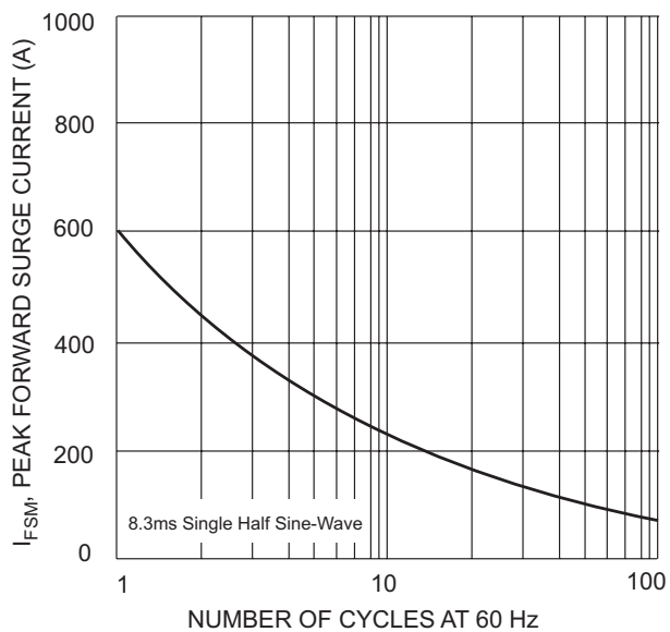
Fig. 3 Maximum Non-Repertive Peak Forward Surge Current
