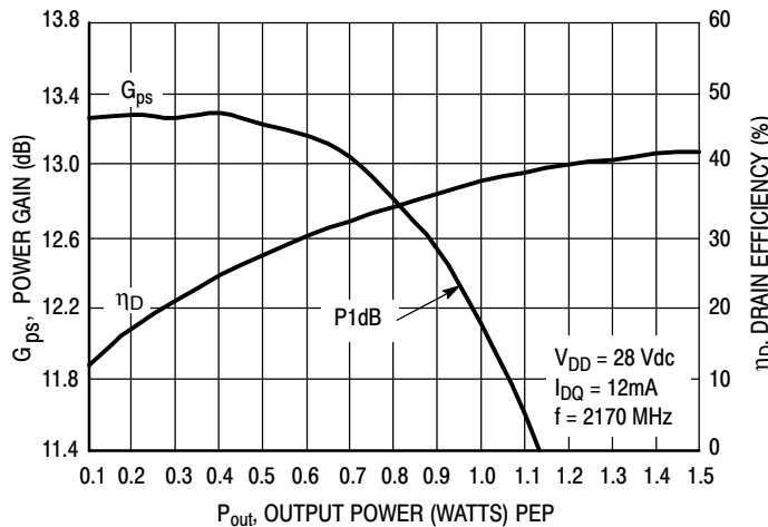
Figure 18. CW Performance versus Output Power
