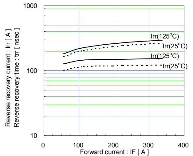
Reverse recovery characteristics (typ.) V_{CC}=600V , V_{GE}=\pm 15V , R_G=3.0\Omega
