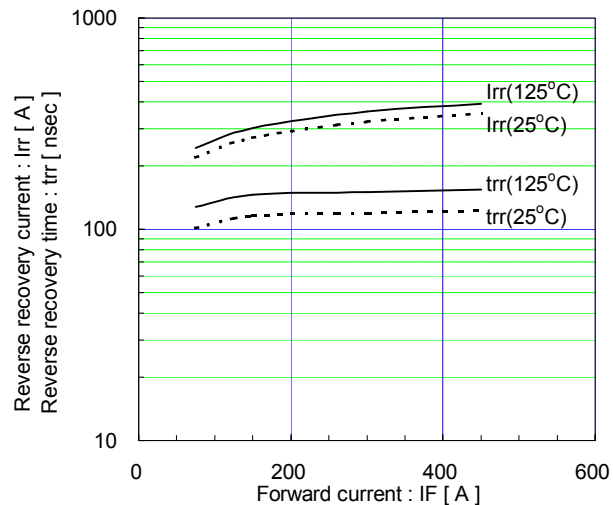
Reverse recovery characteristics (typ.) V_{cc}=600V , V_{GE}=\pm 15V , R_G=2.0\Omega
