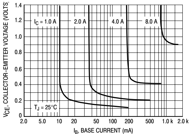
Figure 4. Collector-Saturation Region
