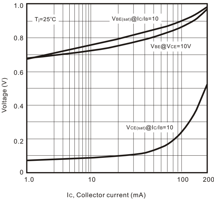
Fig.2 "ON" Voltages
