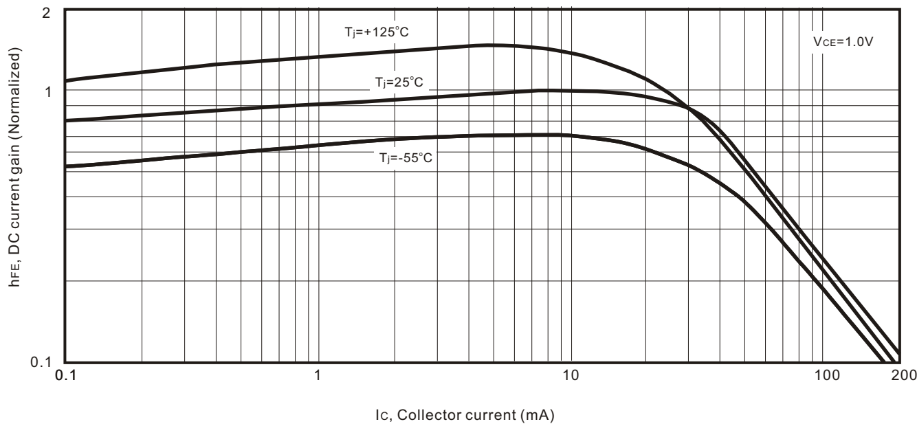
Fig.1 DC current gain
