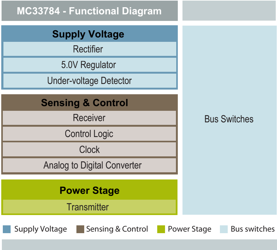
Functional Internal Block Diagram
