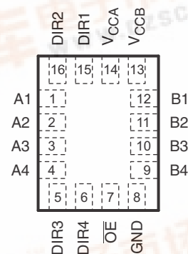
RSV PACKAGE (TOP VIEW)
