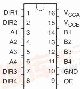
PW PACKAGE (TOP VIEW)
