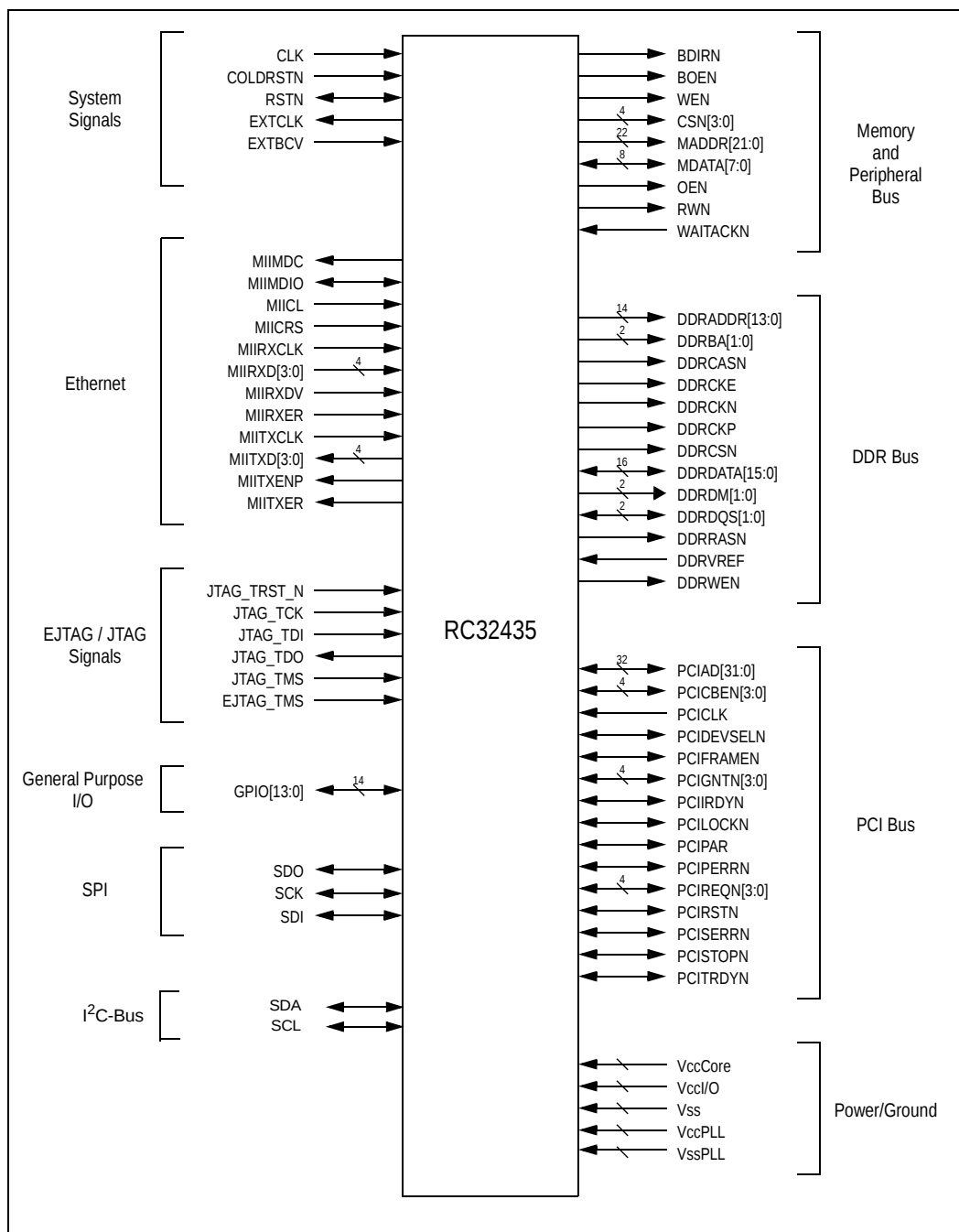
Figure 1 Logic Diagram
