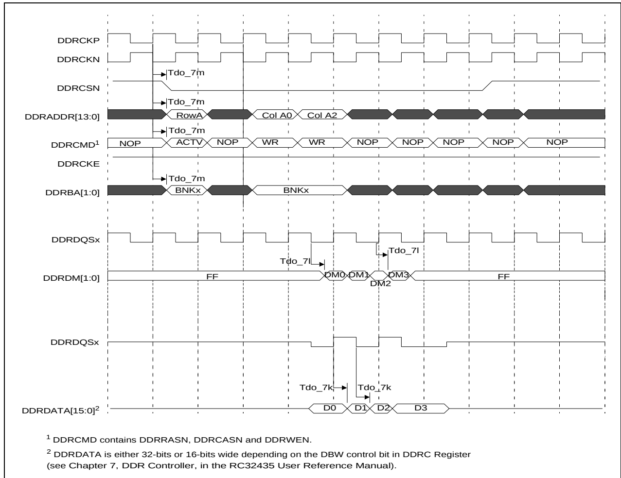
Figure 7 DDR SDRAM Timing Waveform — Write Access
