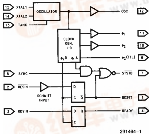
Figure 1. Block Diagram
