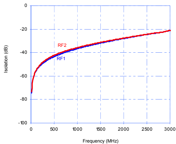
Figure 9. Isolation – RF1 to RF2, RF2 to RF1
