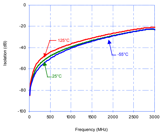
Figure 8. Isolation – RFC to RF2
