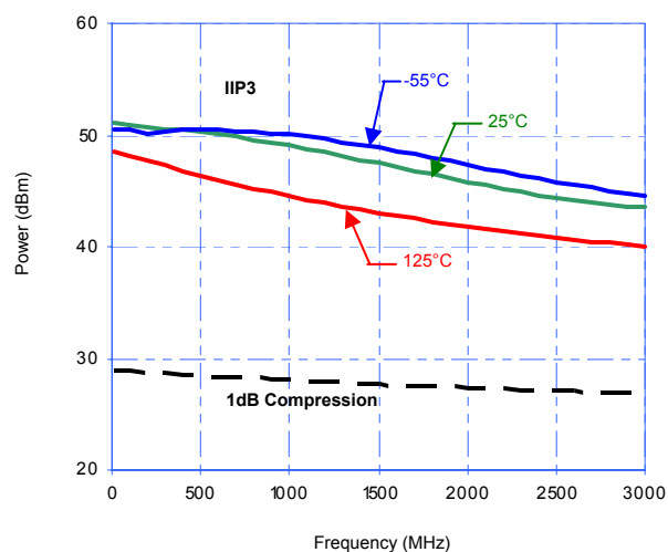
Figure 5. Input 1 dB Compression Point & IIP3
