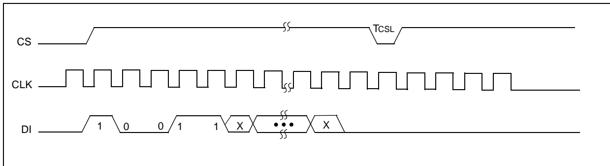
FIGURE 2-3: EWEN TIMING
