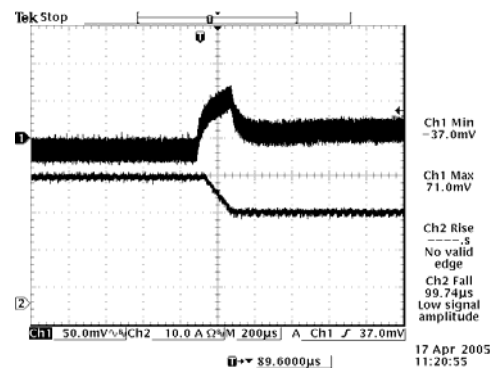
Vout= 1.5 V 75%-50% Load Transients
