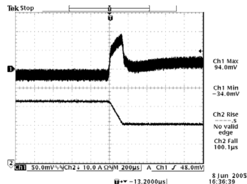
Vout= 1.8 V 75%-50% Load Transients
