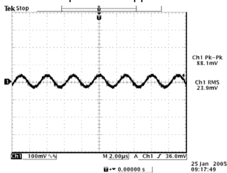
Ripple and noise at full load, 12 V/12 A output
