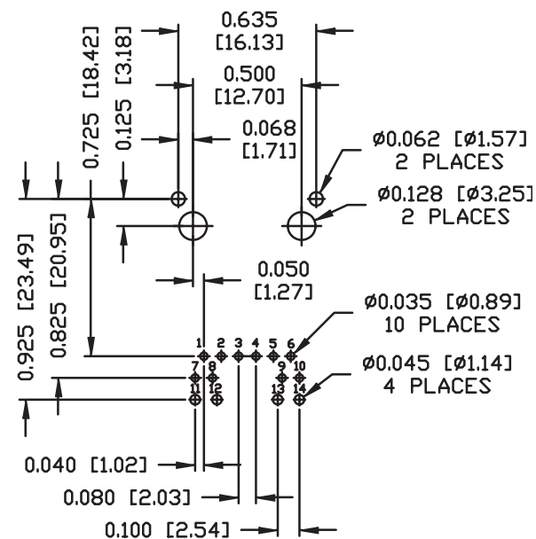
RECOMMENDED PCB FOOTPRINT COMPONENT SIDE VIEW
