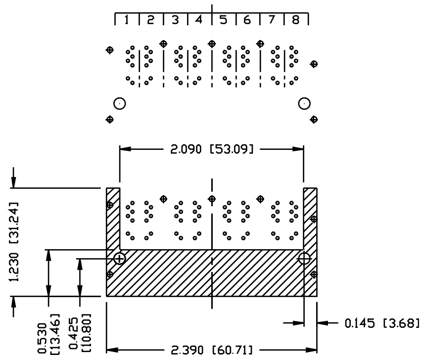
PORT ASSIGNMENT (COMPONENT SIDE VIEW)
