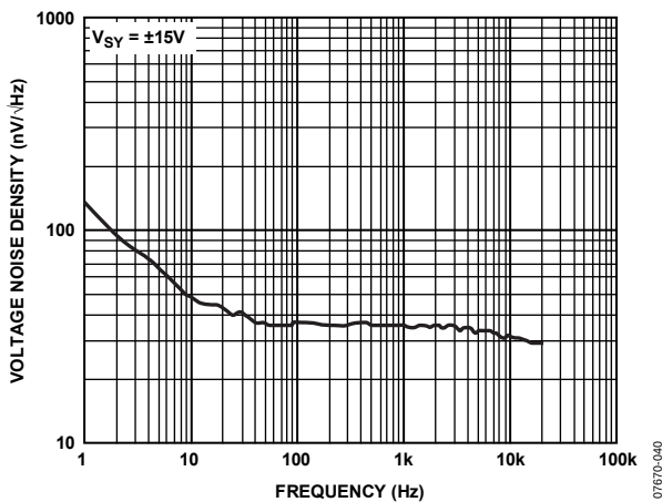
Figure 40. Voltage Noise Density
