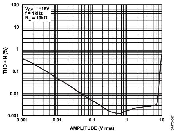
Figure 47. THD + N vs. Amplitude
