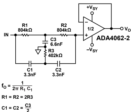
Figure 53. Notch Filter Circuit
