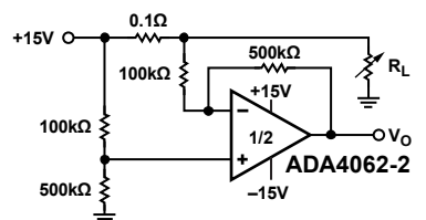
Figure 55. High-Side Signal Conditioning
