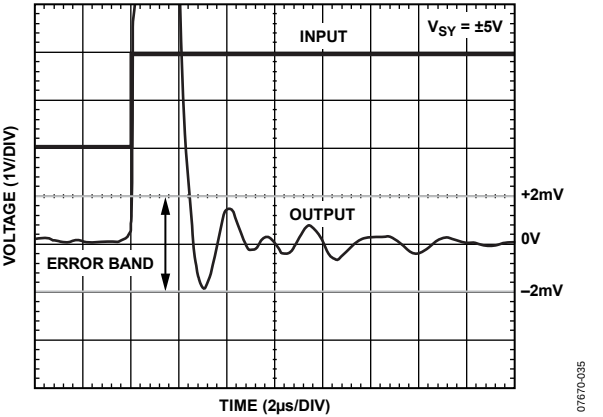
Figure 38. Positive Settling Time to 0.01%
