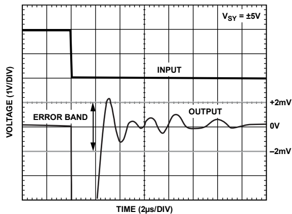
Figure 42. Negative Settling Time to 0.01%
