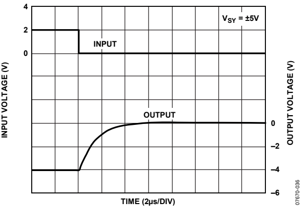
Figure 36. Negative Overload Recovery
