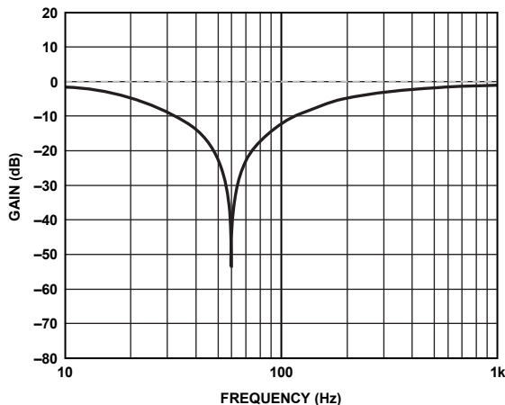
Figure 54. Notch Filter: Gain vs. Frequency
