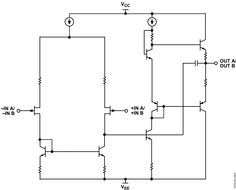
Figure 59. Simplified Schematic
