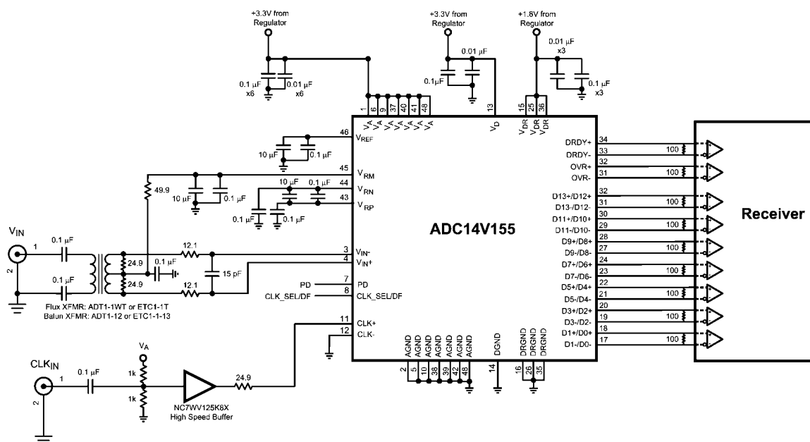
FIGURE 4. Application Circuit using Transformer Drive Circuit
