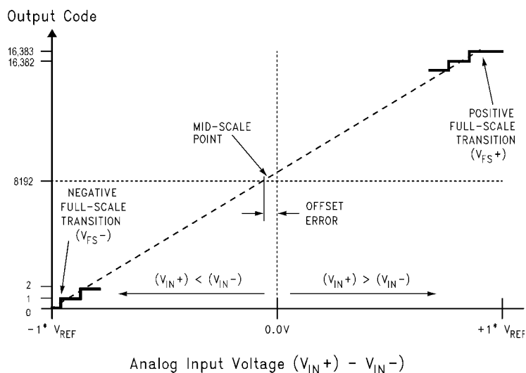
FIGURE 1. Transfer Characteristic (Offset Binary Format)
