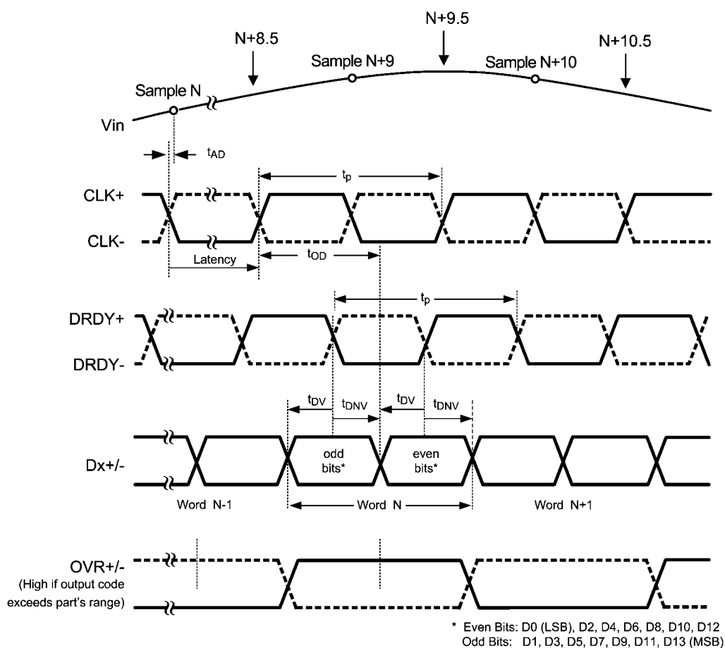
Output Timing
