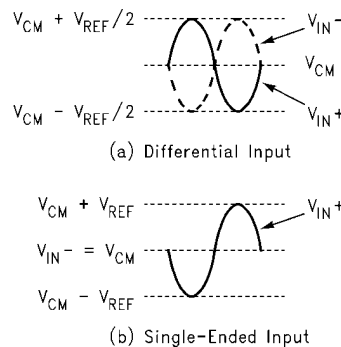
FIGURE 3. Expected Input Signal Range
