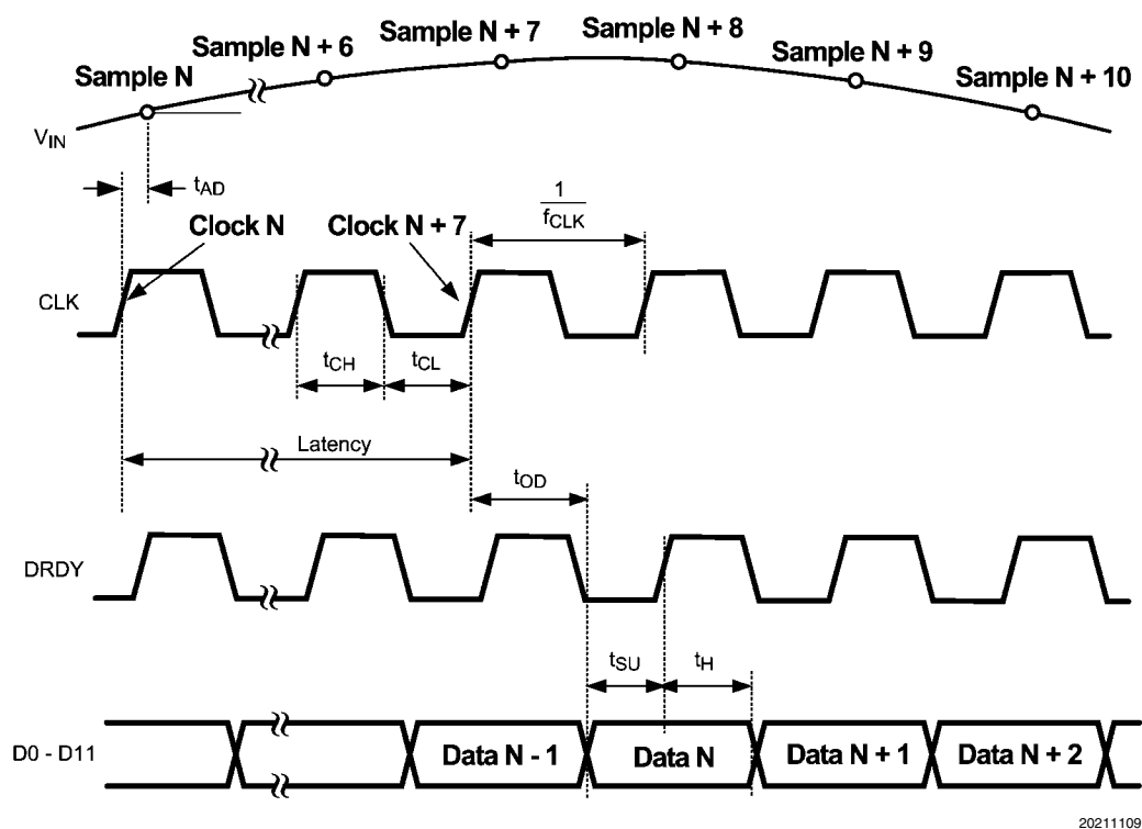
FIGURE 1. Output Timing
