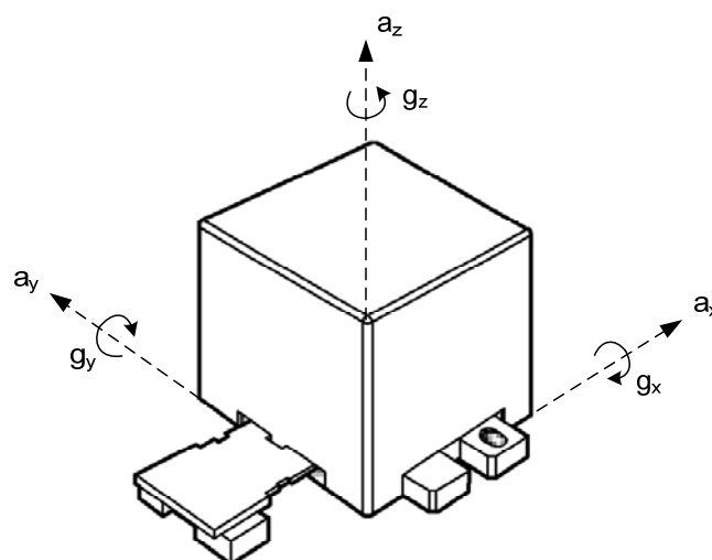
Figure 6. Axial Orientation
