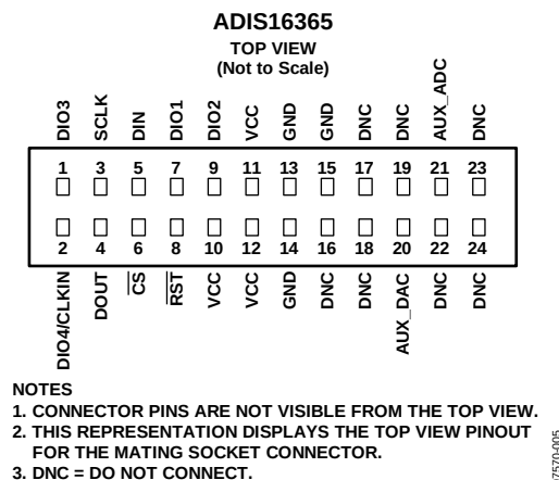
Figure 5. Pin Configuration
