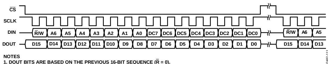
Figure 11. Output Register Bit Assignments
