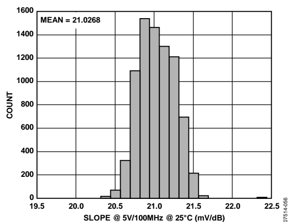
Figure 23. Slope Distribution, 100 MHz
