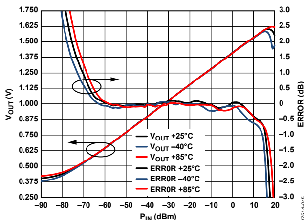
Figure 45. Output and Conformance for the AD8368/ADL5513 Extended Dynamic Range Circuit
