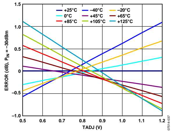
Figure 37. Error vs. V_{TADJ} , P_{IN} = -30 dBm at 1900 MHz
